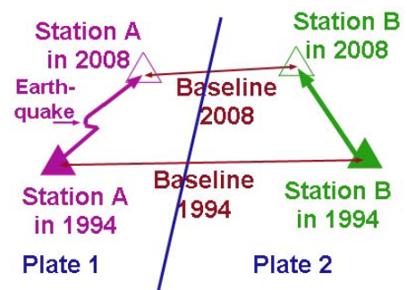
Figure 3. Effect of tectonic deformation on coordinates & baselines
